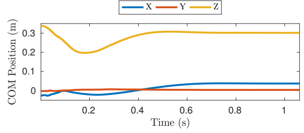
(a) COM Position
