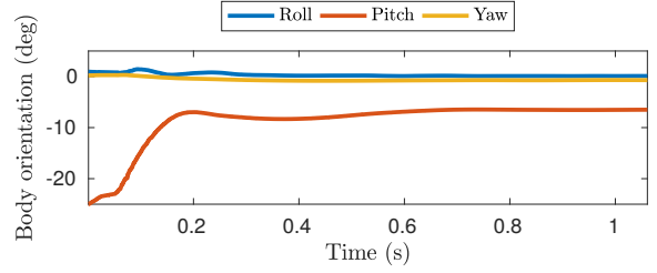
(b) Body Orientation
