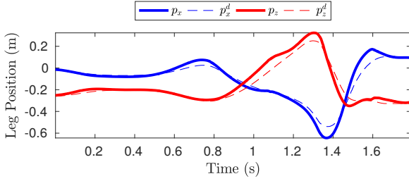
(c) Back-right leg position
