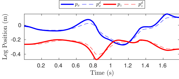
(a) Front-right leg position
