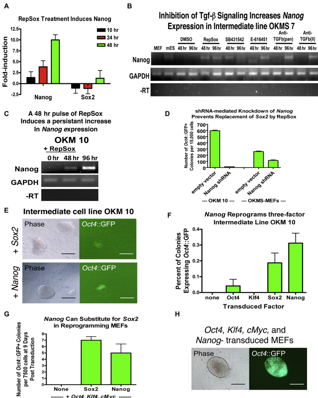
Figure 6. RepSox Replaces Sox2 by Inducing Nanog Expression
