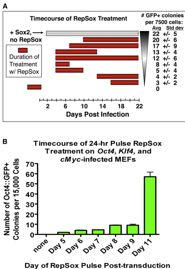
Figure 4. A Short Pulse of RepSox Is Sufficient for Sox2 Replacement and Most Effective at Later Time Points after Infection
