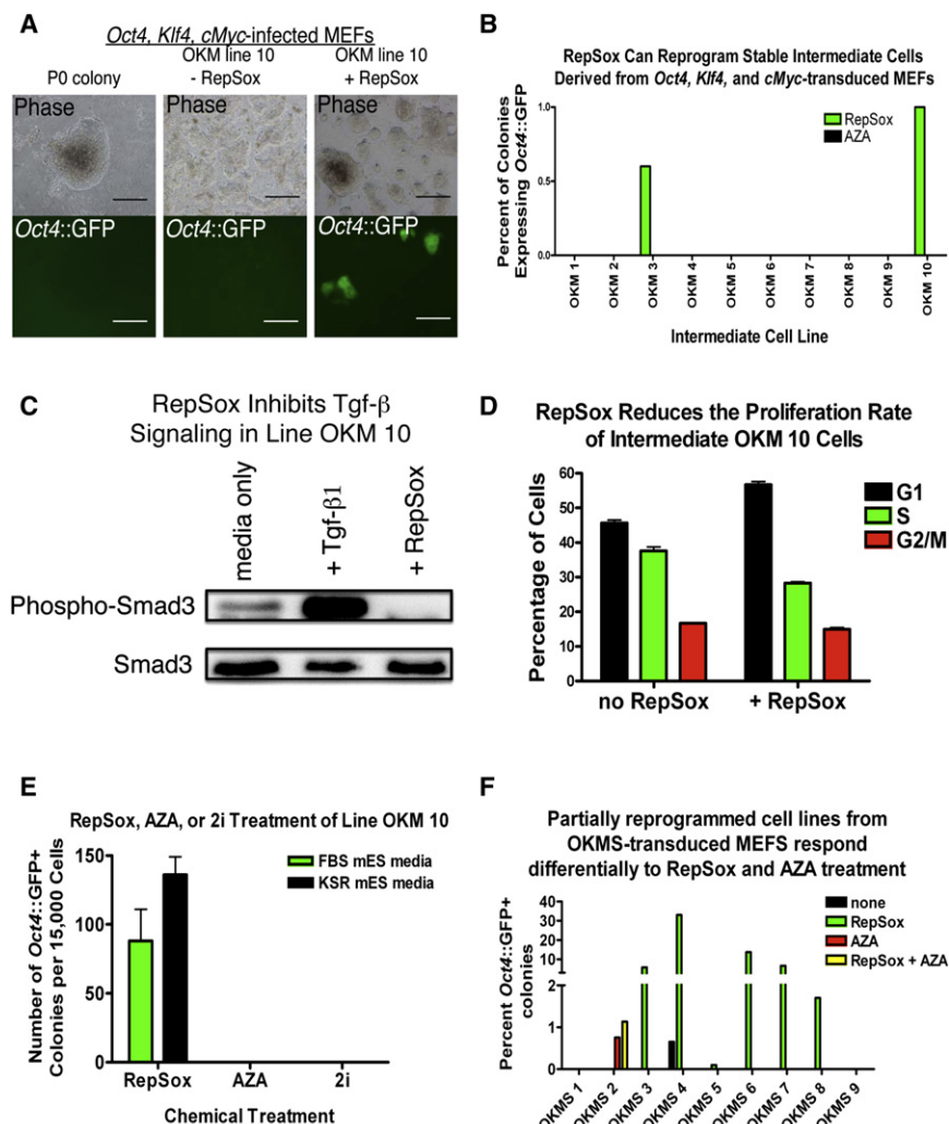
Figure 5. Stable Intermediates Can Be Reprogrammed by RepSox
