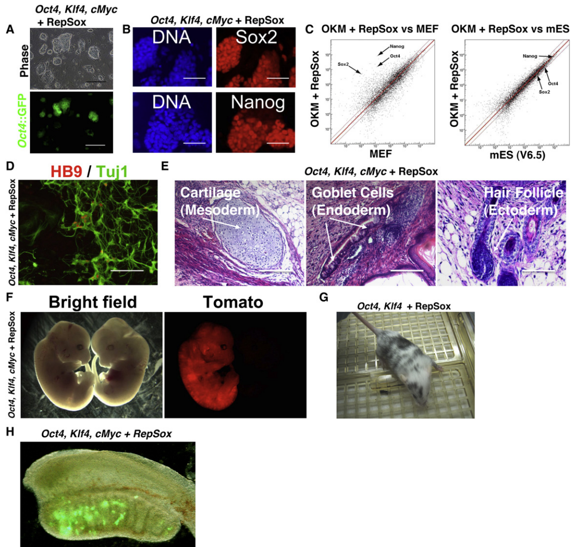
Figure 2. RepSox-Reprogrammed Cells Are Pluripotent
