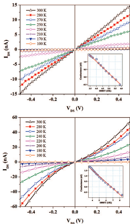
Figure 6. I – V curves of (a) \text{Zn}_3\text{P}_2 and (b) \text{Cd}_3\text{P}_2 nanobelts measured at 300–100 K. The insets show the conductance in a logarithmic scale at zero bias voltage plotted as a function of 1000/T .
