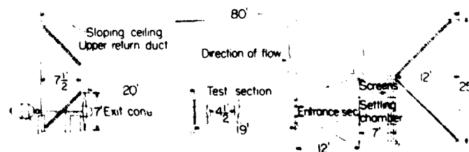
FIGURE 1. Elevation view of 4½-foot wind tunnel.
