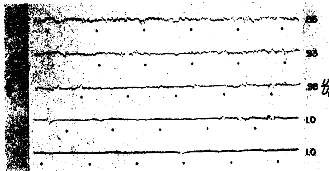
FIGURE 17.—Turbulence velocity \omega_z in boundary layer. U_1 , 50 feet per second; timing dots, 60 per second.
