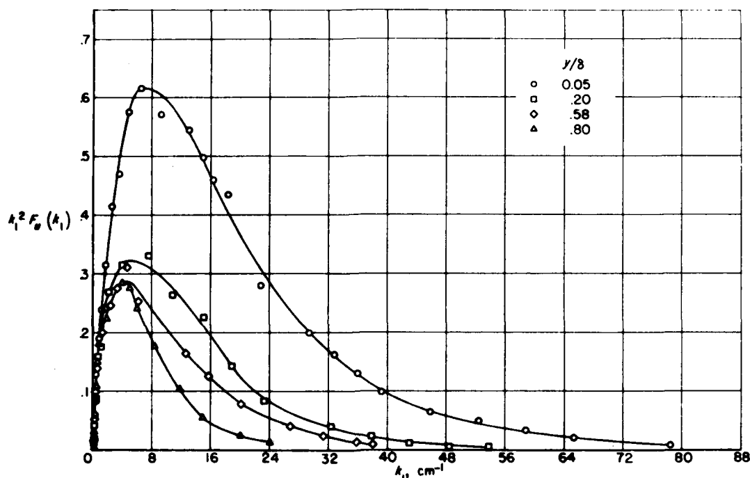
FIGURE 26.-- Second moment of \bar{u}^2 spectra.
