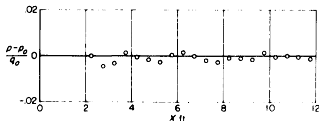
FIGURE 2. Pressure distribution along flat plate.
