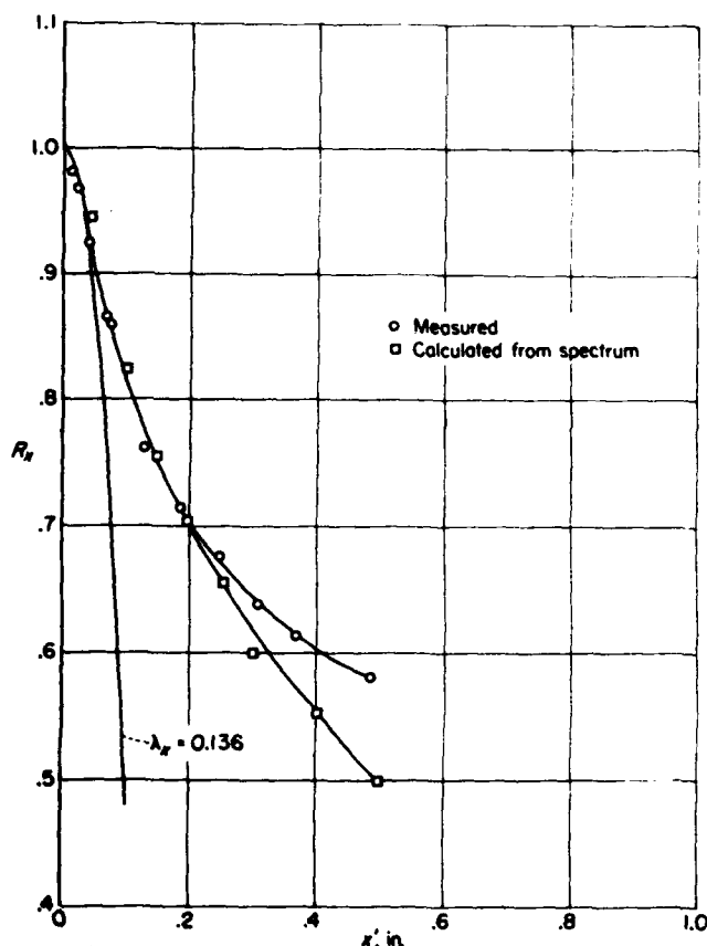
FIGURE 15. Comparison of longitudinal correlation coefficient R_x obtained directly with that calculated from spectrum of \bar{u}^2 ; y/\delta = 0.05 . Curve for \lambda_x also calculated from spectrum.
