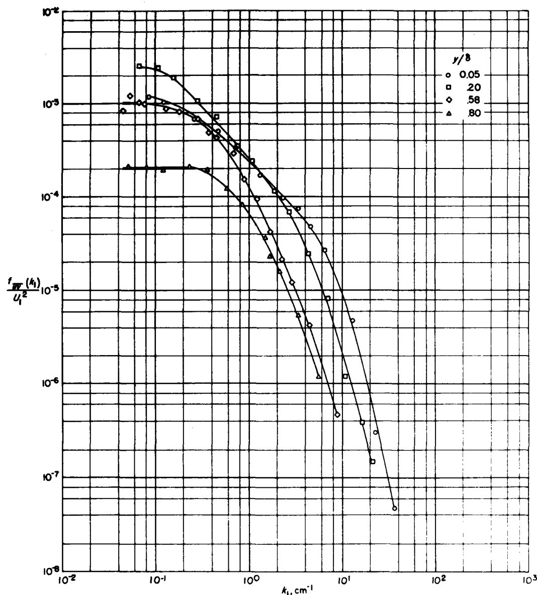
FIGURE 8.—Spectra of turbulent shear stress.
