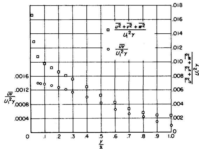
FIGURE 20.—Turbulent shear stress and turbulent energy divided by \gamma .
