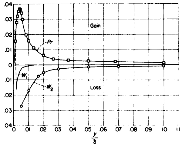
FIGURE 23. Production and dissipation in region near wall.
