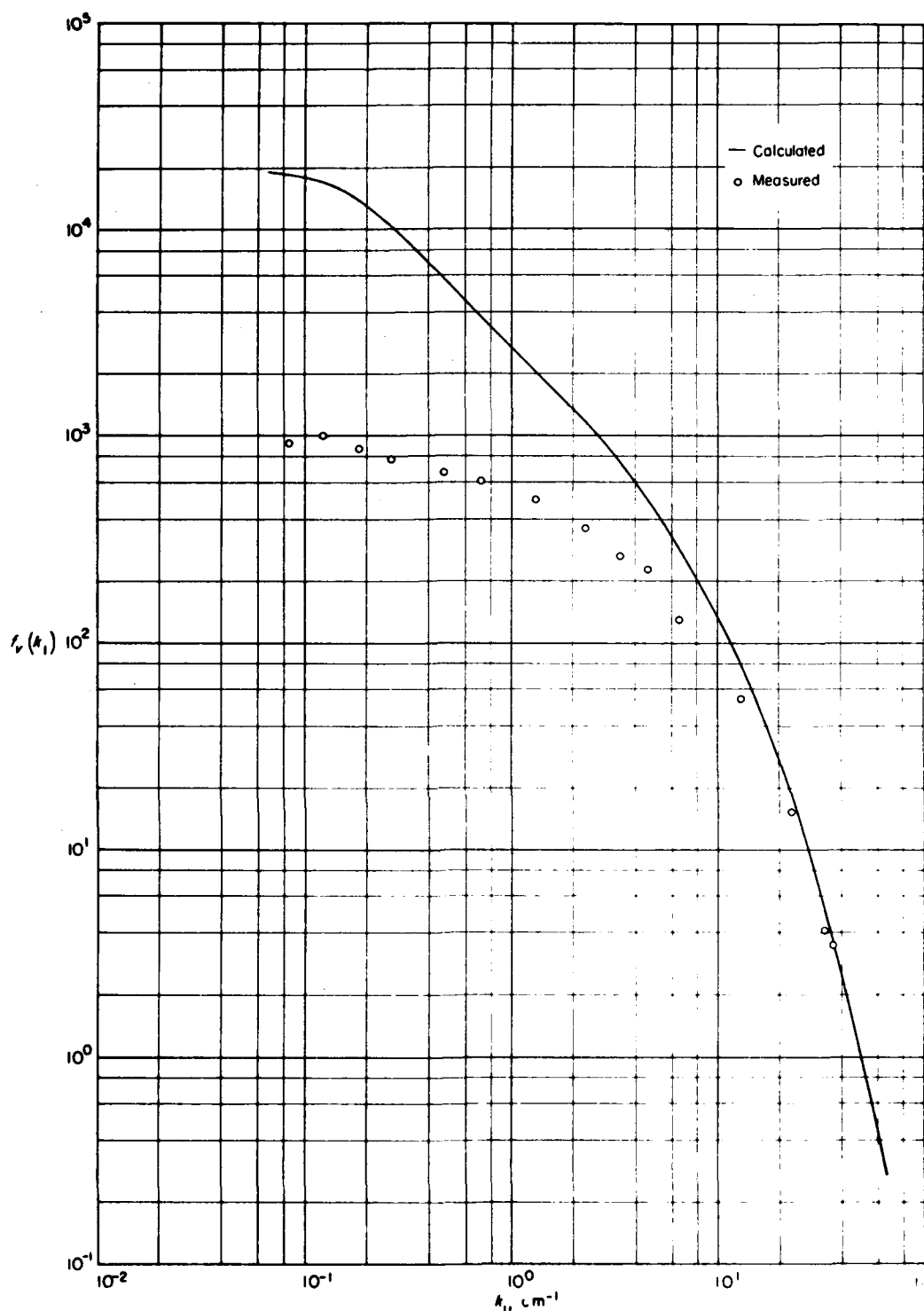
FIGURE 9—Comparison of measured \overline{v^2} spectrum with that calculated from measured \overline{u^2} spectrum using isotropic relation; u/\delta = 0.05
