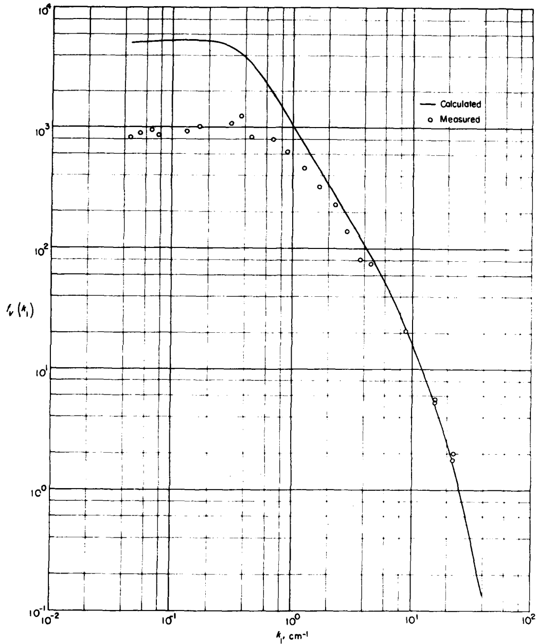
FIGURE 10. Comparison of measured \overline{w^2} spectrum with that calculated from \overline{u^2} spectrum using isotropic relation; y/\delta = 0.58 .
