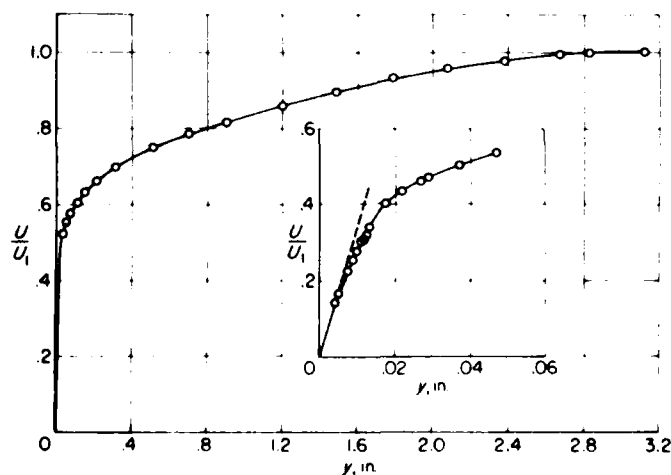
FIGURE 3. Mean velocity distribution
