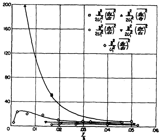
FIGURE 13.—Distribution of dissipation derivatives near wall.
