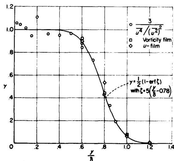
FIGURE 18.—Distribution of intermittency factor.
