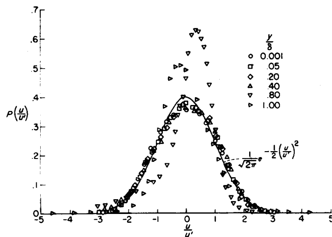
FIGURE 11.—Distributions of probability density.
